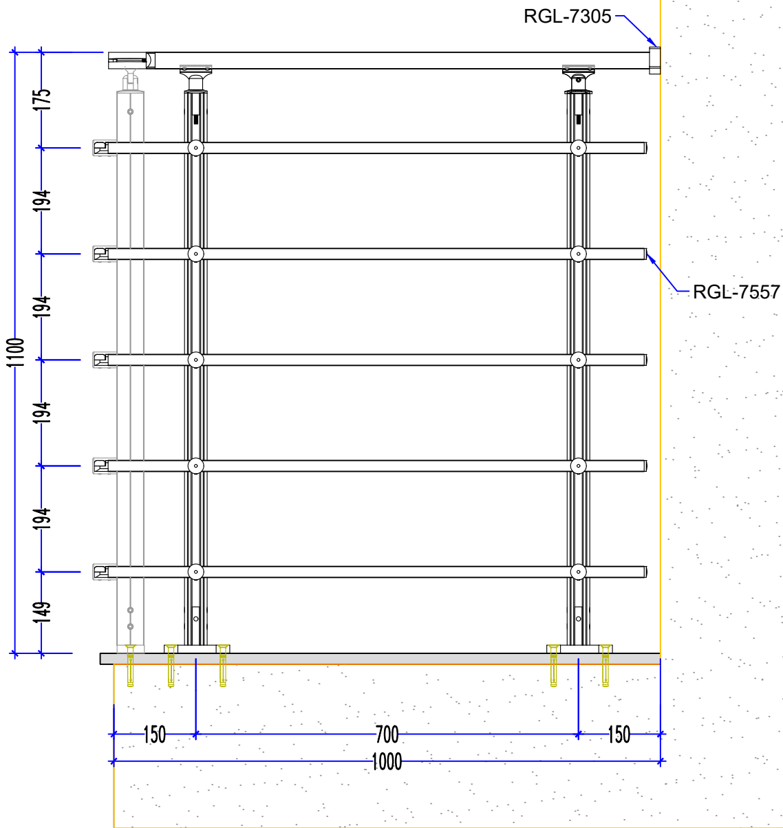
RIGHT VIEW
