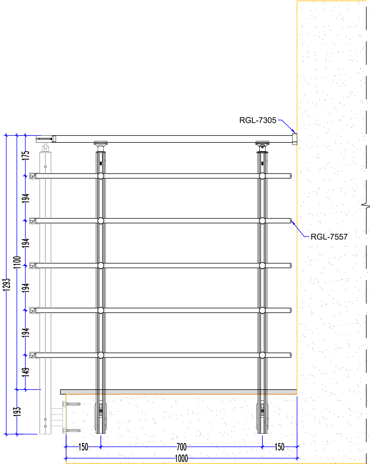
RIGHT VIEW
