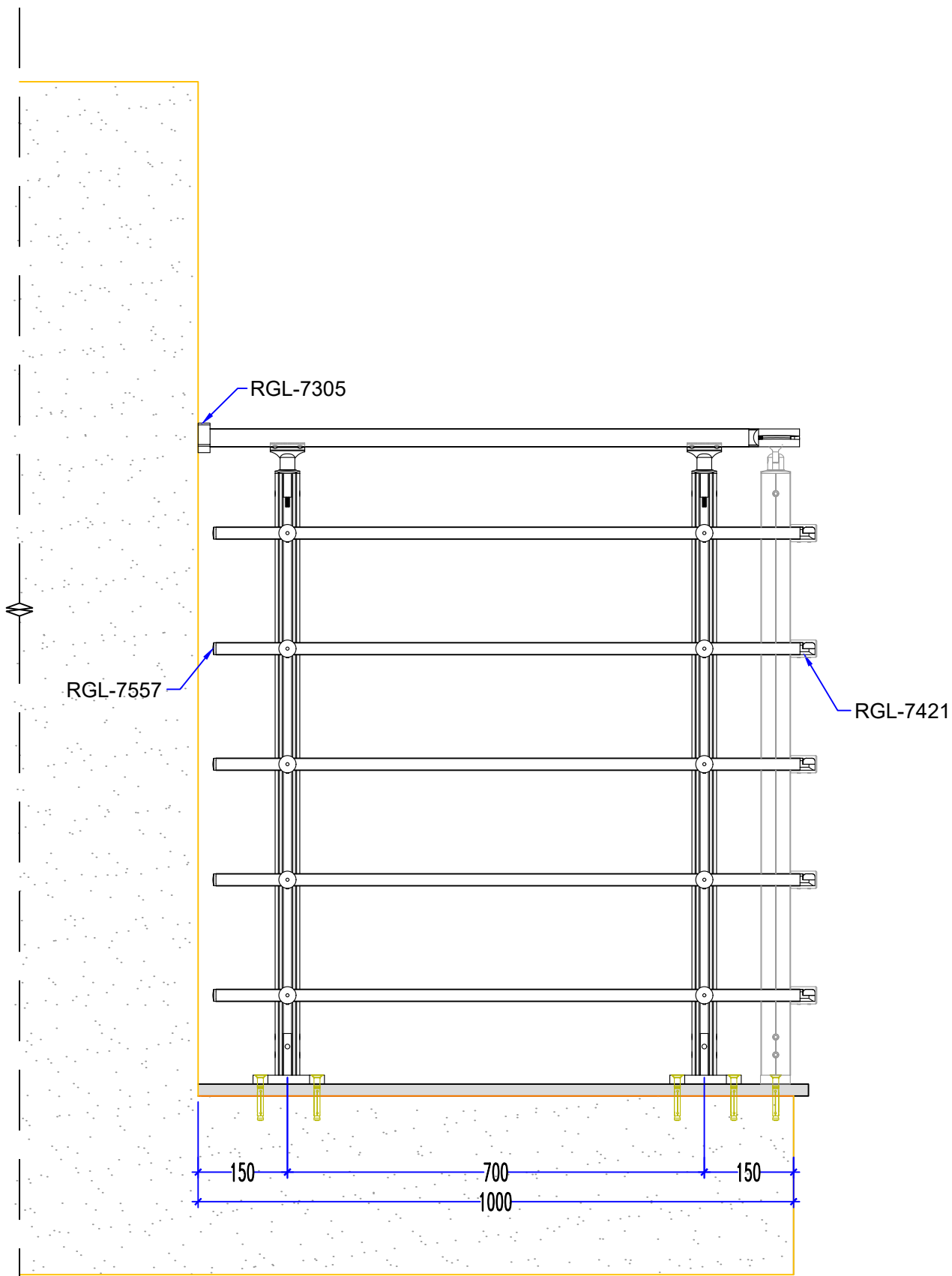
RIGHT VIEW
