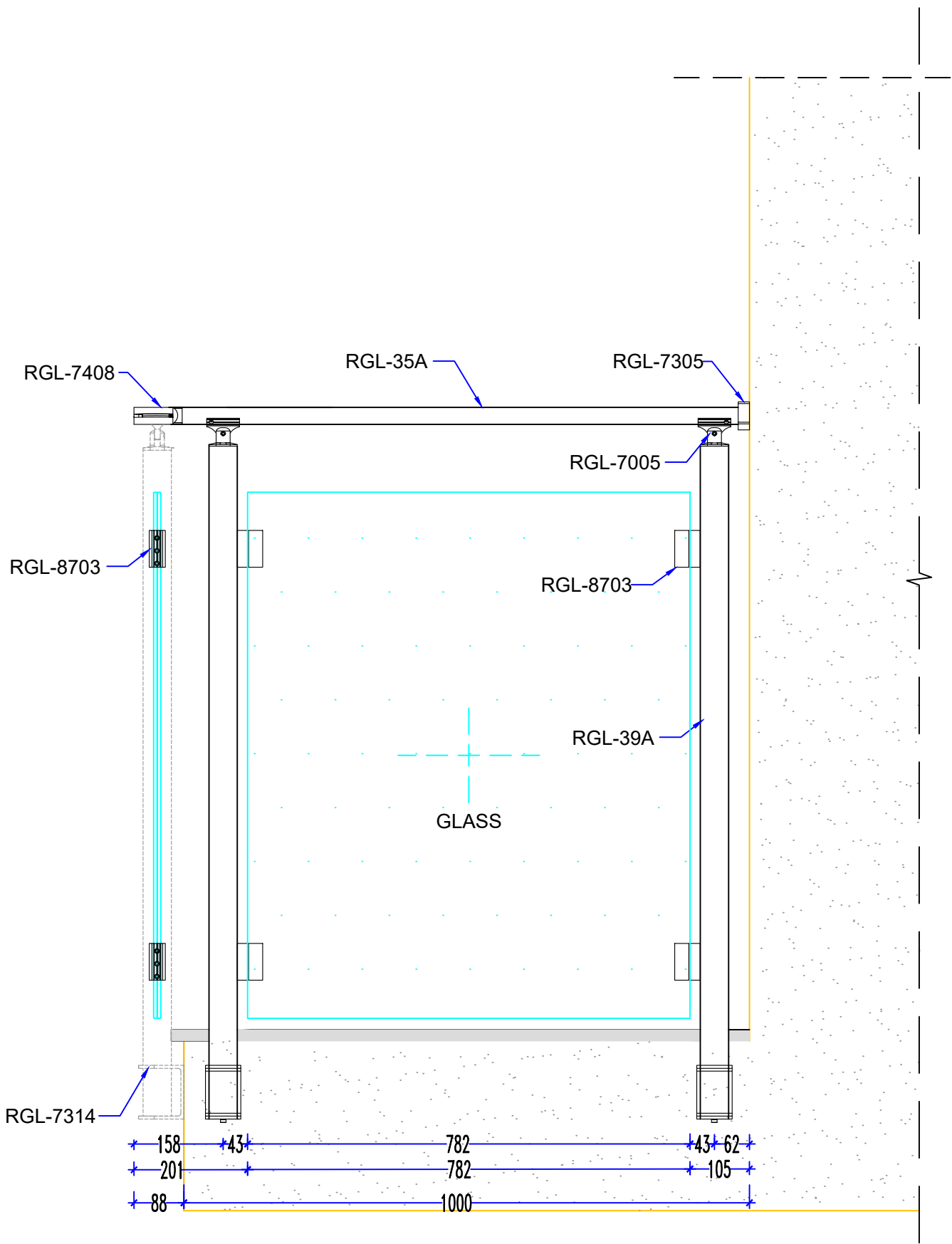
RIGHT VIEW
