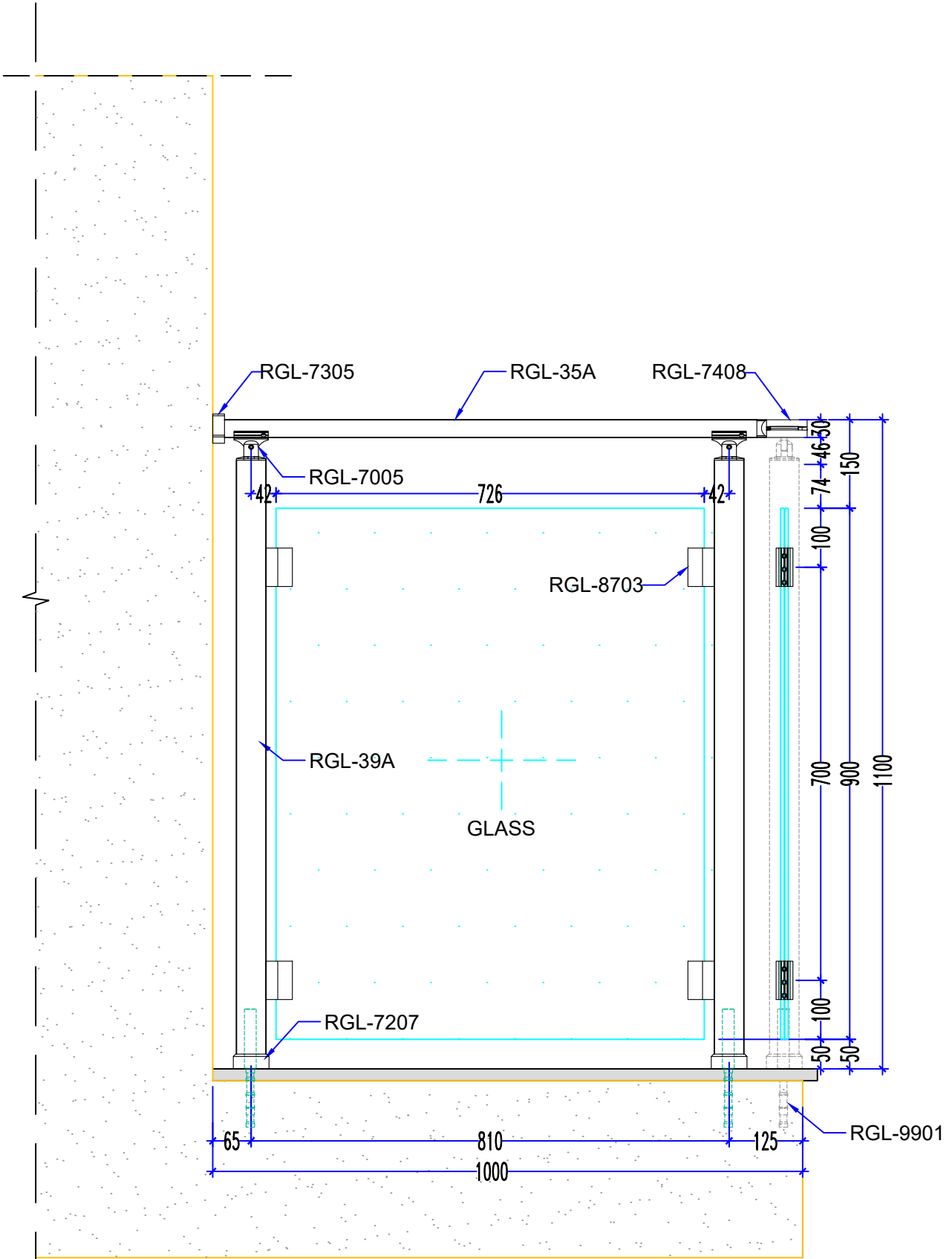
LEFT VIEW
