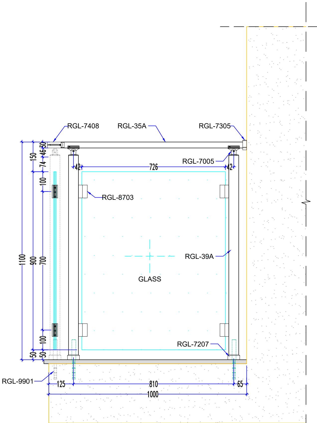
RIGHT VIEW
