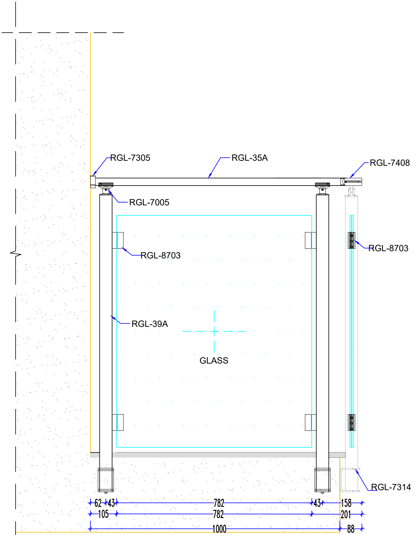
LEFT VIEW
