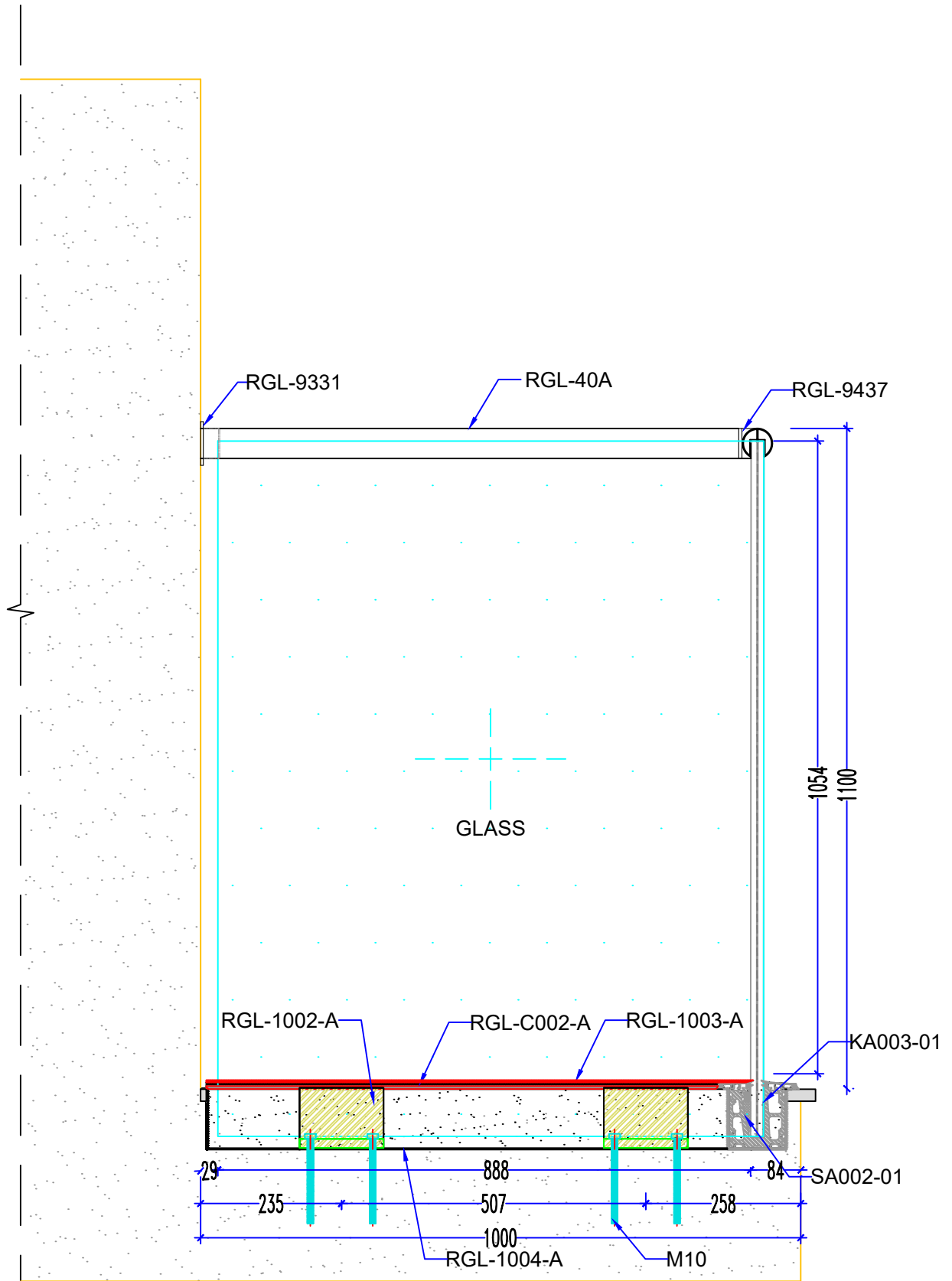
LEFT VIEW
