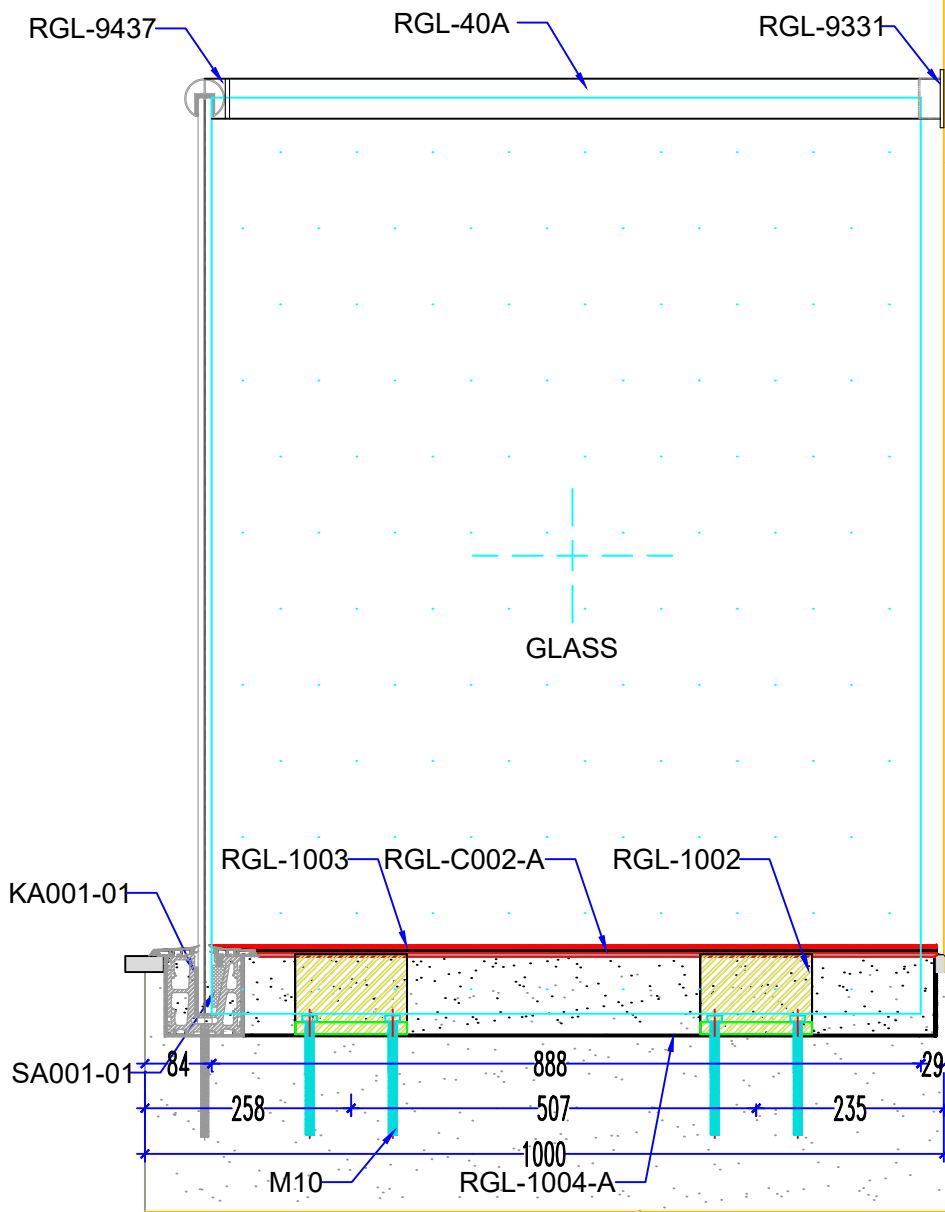
RIGHT VIEW
