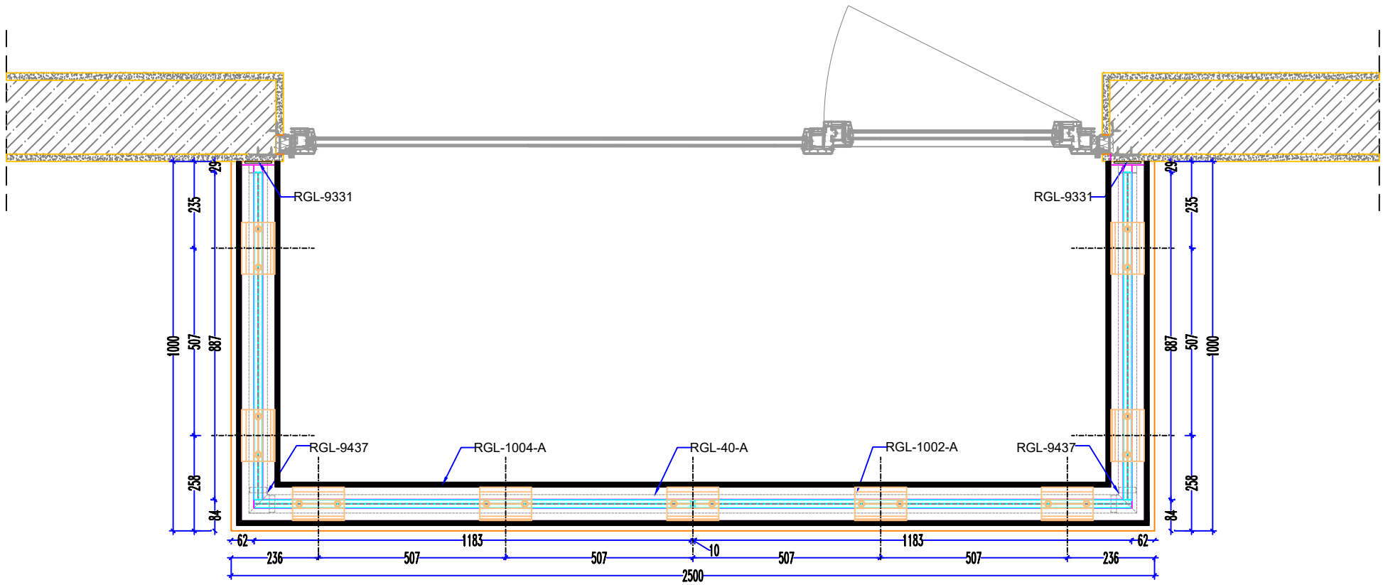
PLAN
