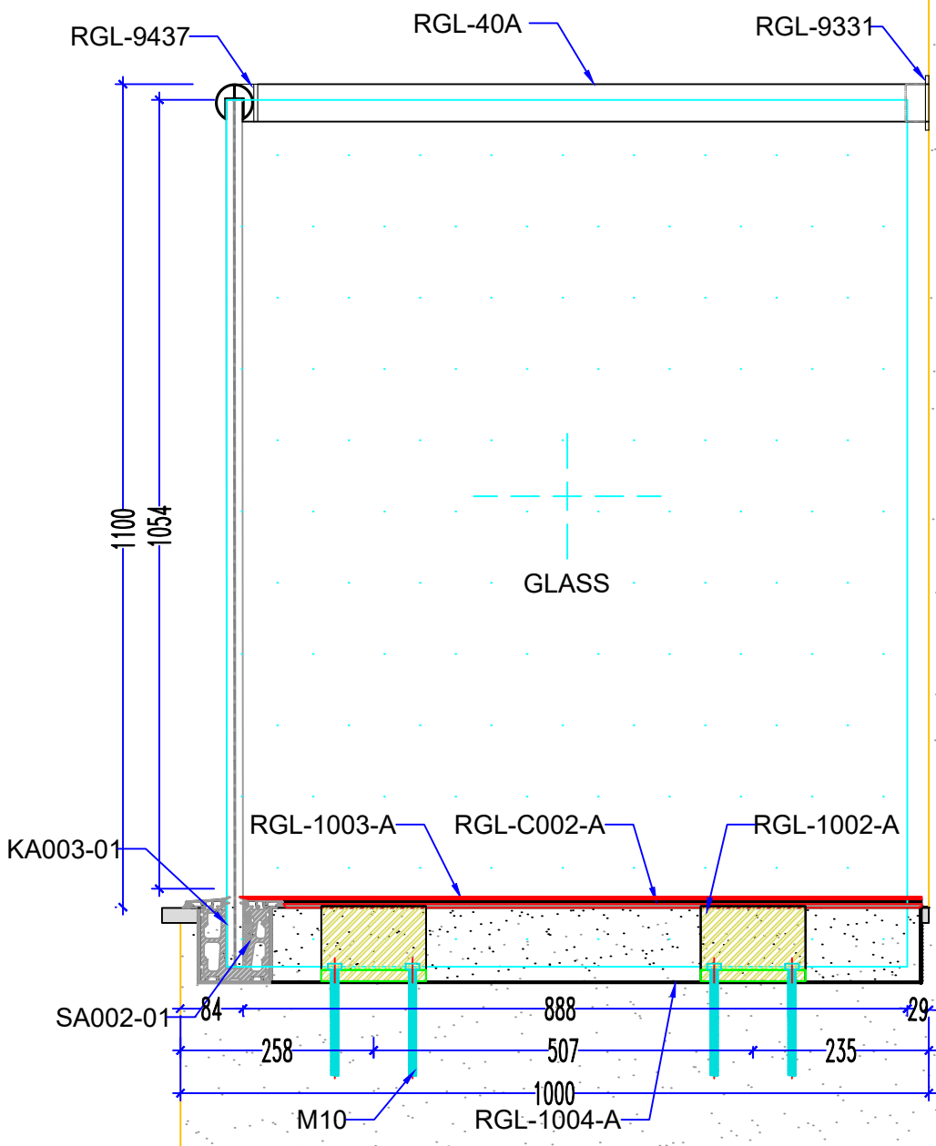
RIGHT VIEW
