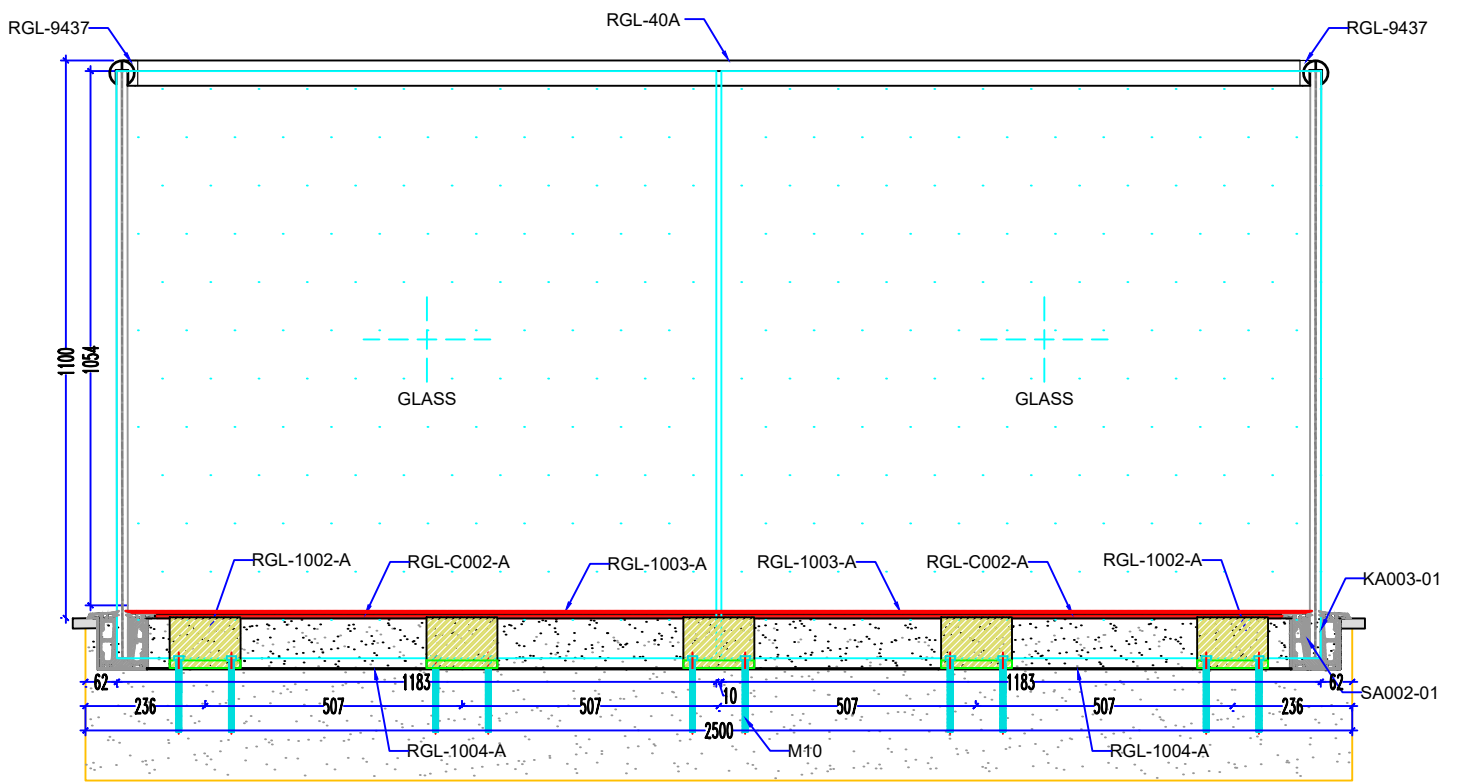
FRONT VIEW
